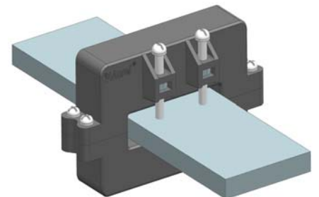
Base Plate Screw M4 (gasket) Installation
